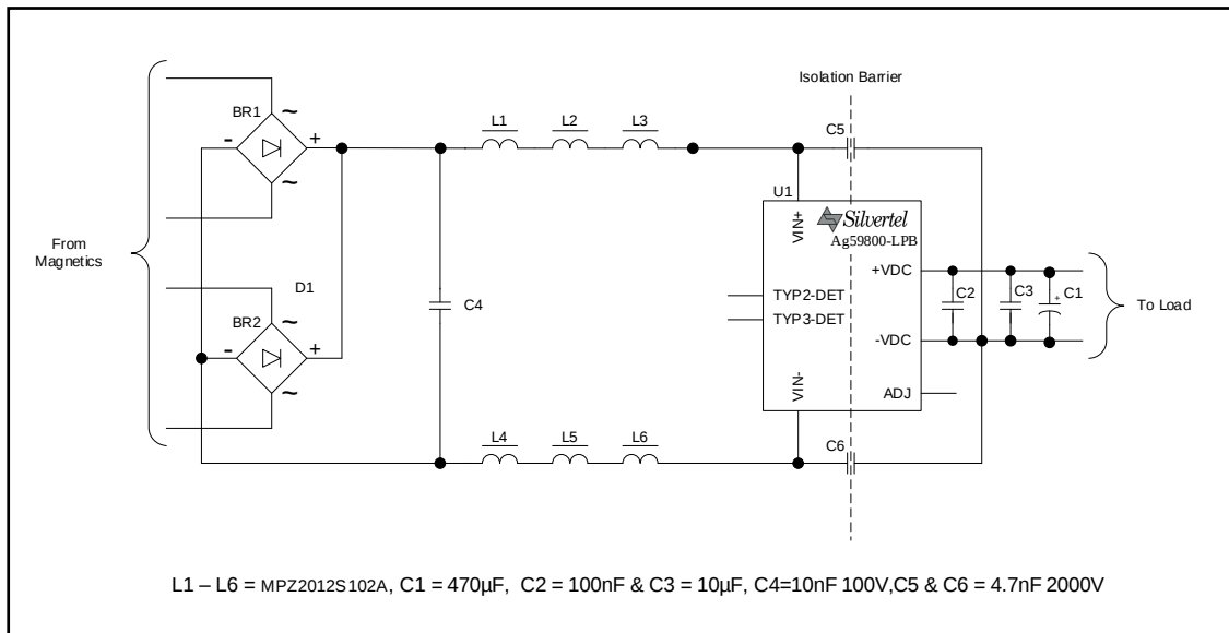
Figure 12: Typical Connection Diagram
