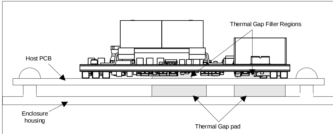
Figure 10: Additional Heatsinking
